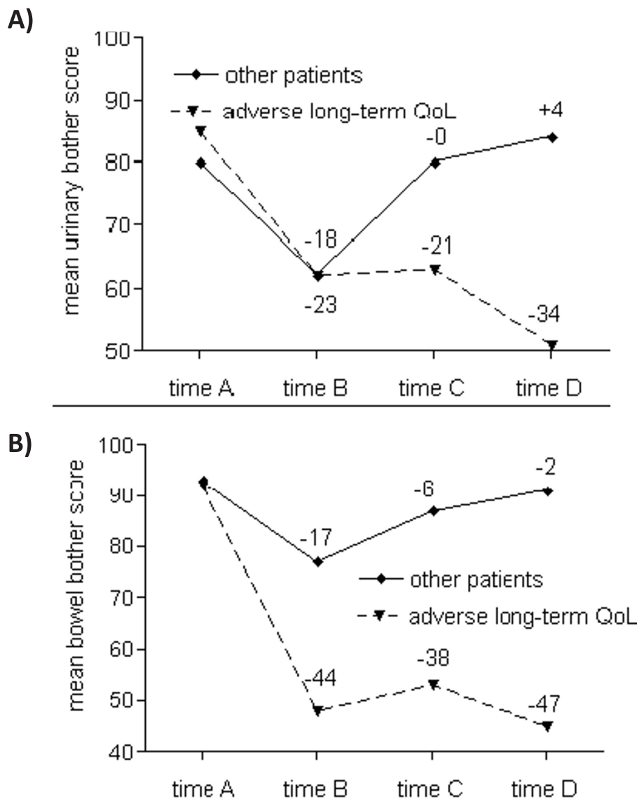
Figure 2 Mean urinary (A) and bowel (B) bother scores for patients with vs. without adverse long-term urinary quality of life (QoL).
