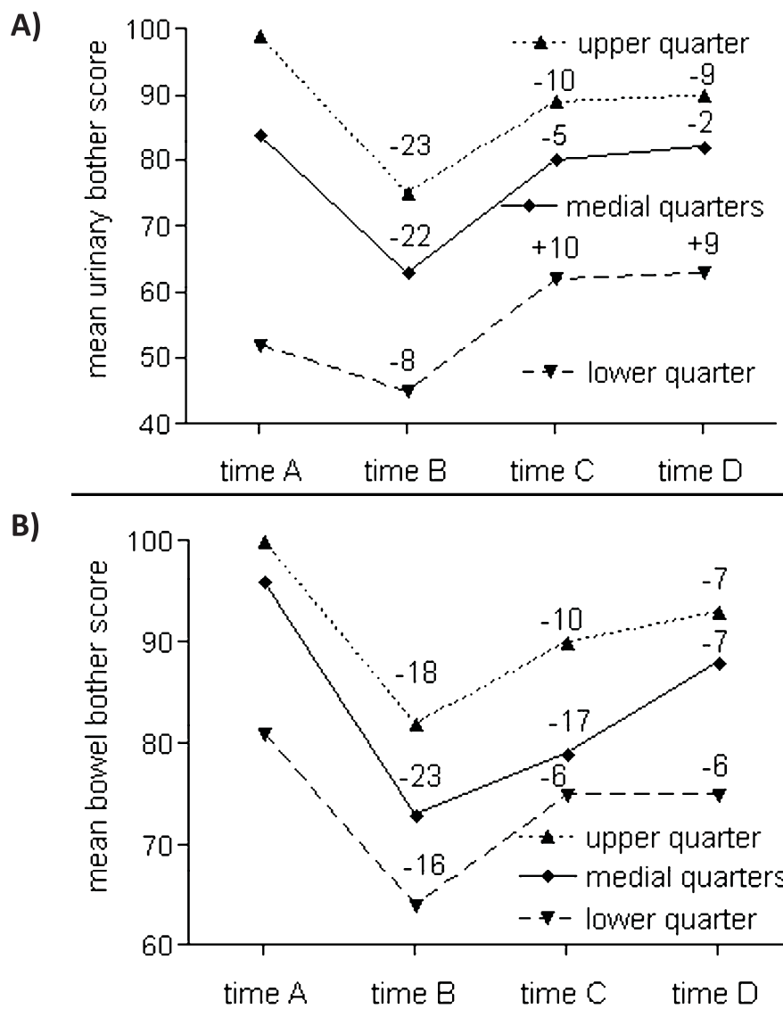
Figure 1 Mean urinary (A) and bowel (B) bother scores in dependence on the baseline scores. A: Baseline score for lower quarter: <70; medial quarter: 70-95; upper quarter: >95. All changes statistically significant ( p < 0.05 ), except changes at time D for patients in the medial quarter. B: Baseline score for lower quarter: <93; medial quarter: 93-99; upper quarter: 100. All changes statistically significant ( p < 0.05 ).
